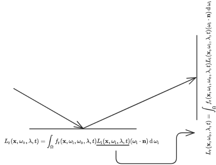
Figure 2: A Recursive Application of the Rendering Equation
